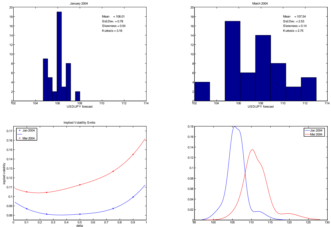
Figure 1: Beliefs, implied volatility smiles, and risk-neutral densities. The first and second plot show histograms of the one-month foreign exchange forecasts for the USD/JPY at the beginning of January 2004 and March 2004. The plots also report the mean, standard deviation, skewness and kurtosis of the forecasts. The third panel is the cubic-spline interpolated implied volatility of one-month currency options as a function of the delta for January and March 2004. The fourth panel shows the option-implied state price density of the USD/JPY in January and March 2004.
